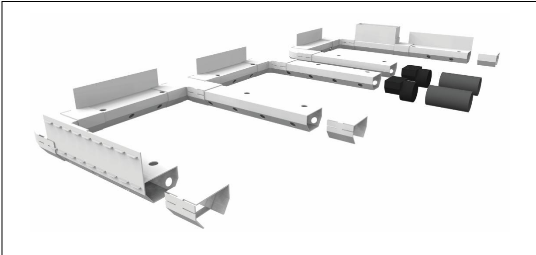
Figure 1 Newton Basedrain (all dimensions in mm)
